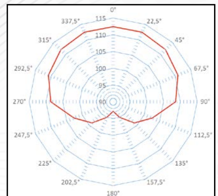
Controlled cardioid dispersion pattern
